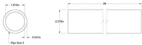
Some material and part specifications. Weights, connection points, weather/wind proofing etc
